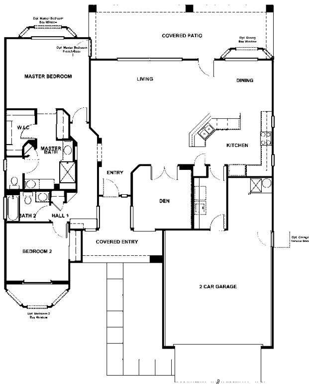
San Dimas 1,678 square feet
