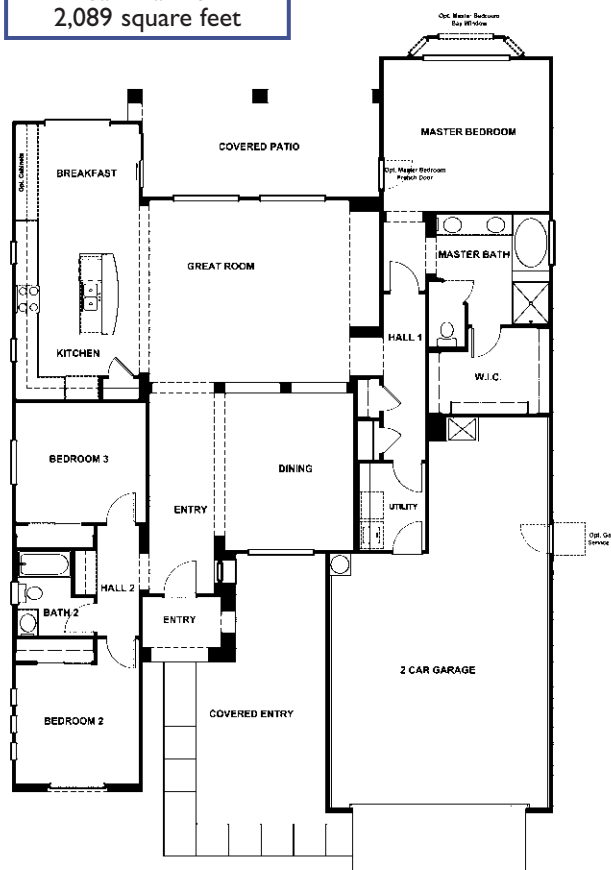
San Marino 2,089 square feet
